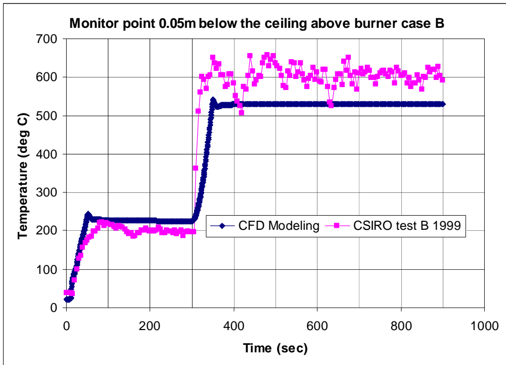
Figure 11: Gas temperature above the burner 0.05m below the ceiling for case B
