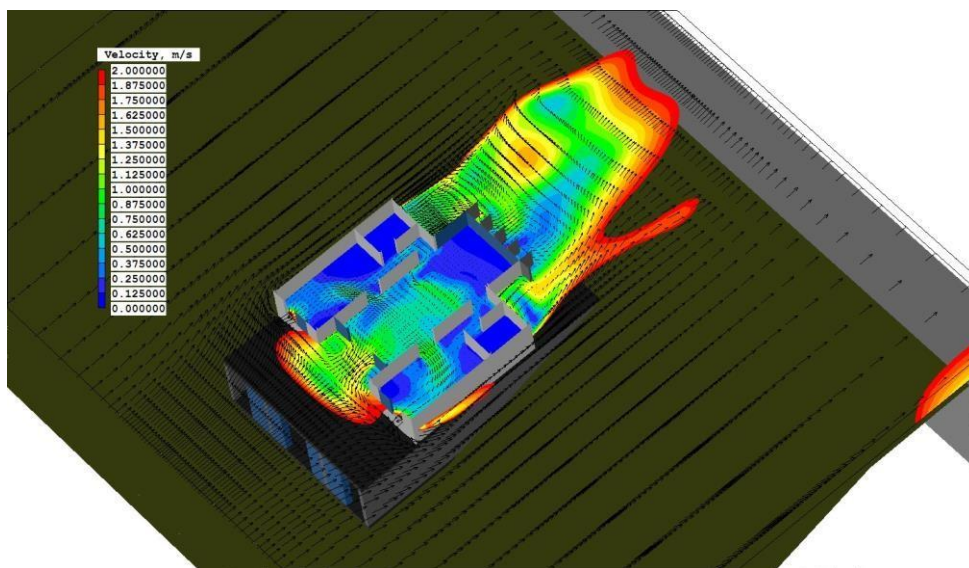
Figure 3. Velocity profile in z-plane
