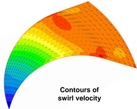
Pressure and swirl velocity contours from 3-D rotor analysis
