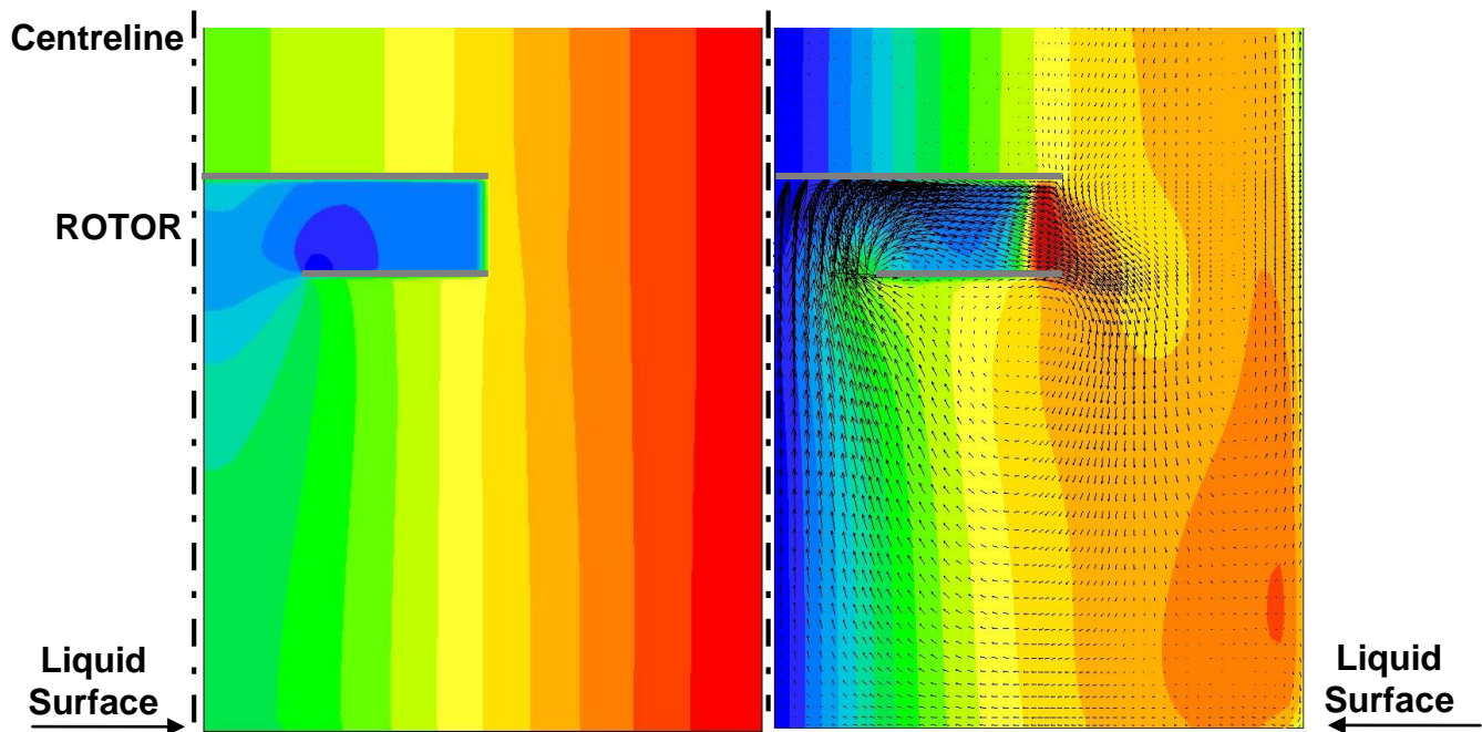
Pressure and swirl velocity contours from 2-D analysis
